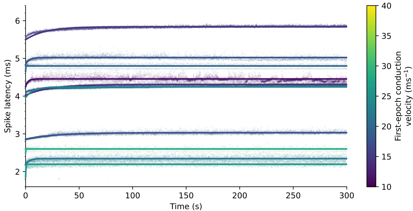
Spike latency and CV changes
